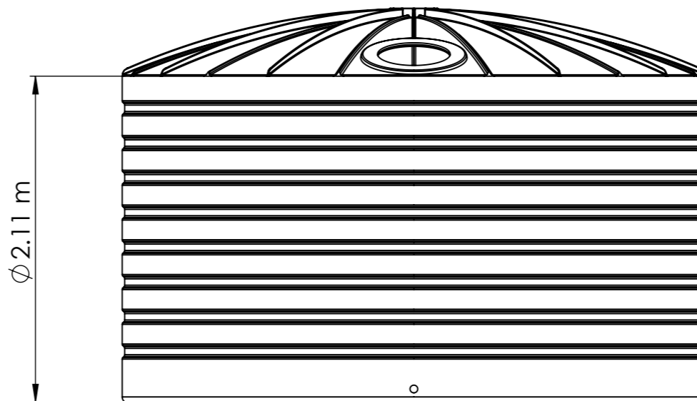
12 FRONT VIEW
